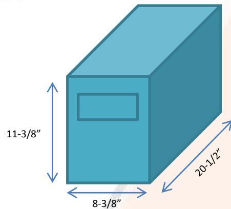
OLD SERIES VENT CUTOUT
