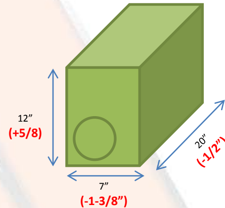
NEW SERIES CUTOUT
