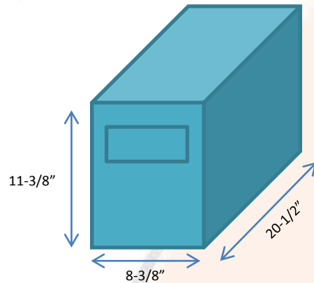
OLD SERIES DIMENSIONS
