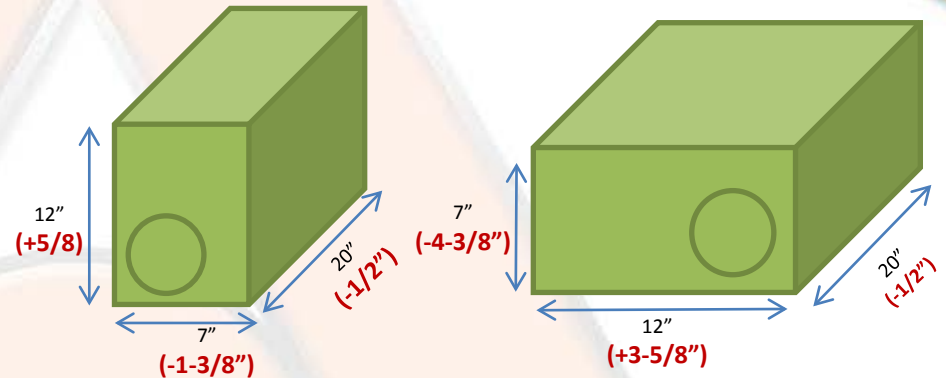
NEW SERIES VENT CUTOUT
