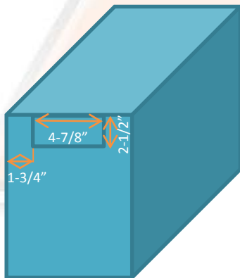
OLD SERIES VENT CUTOUT
