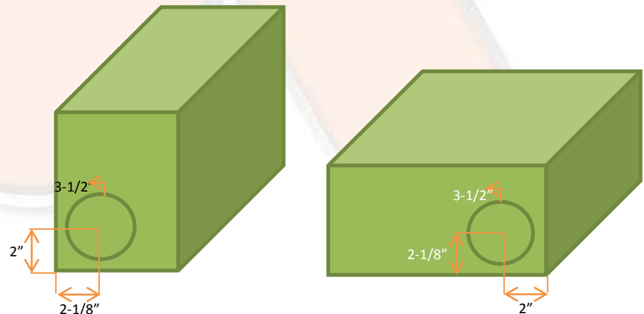
NEW SERIES VENT CUTOUT
