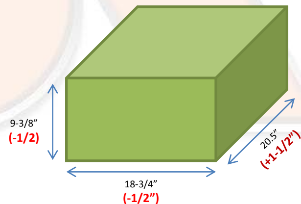
NEW SERIES FLUSH DOOR
